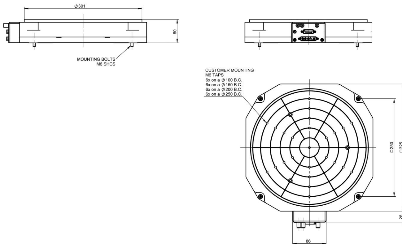
A-637.x100, dimensions in mm
