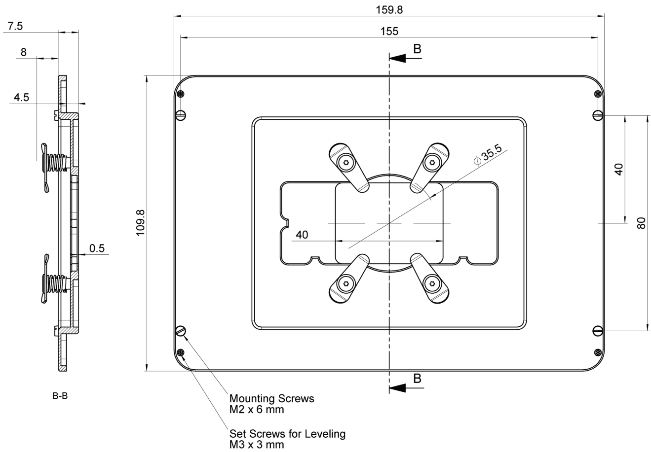
P-736.PDN, Abmessungen in mm
