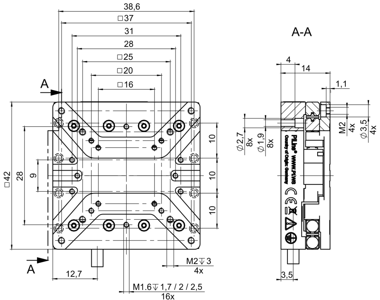
U-523, Dimensions in mm
